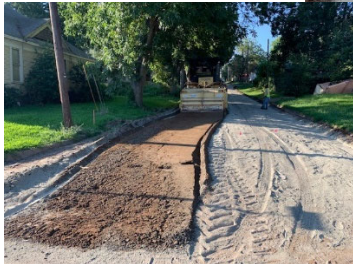
Machine mixing pulverized soil with Portland cement
